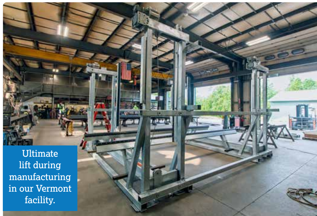
6,000 lb. capacity Ultimate Boat Lift.
