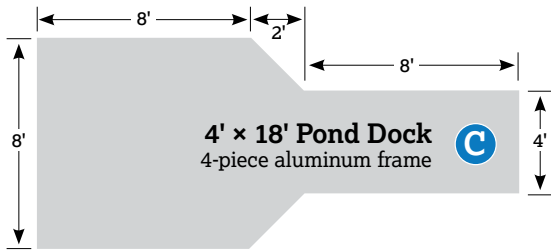
(C) 4' x 18' Pond Dock 4-piece aluminum frame
