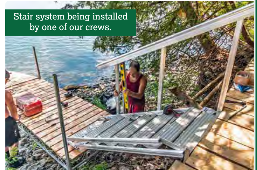
Above: Stair system on an oceanfront property can be easily removed in winter to protect the stairs.
