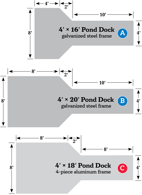
C 4' x 18' Pond Dock 4-piece aluminum frame
