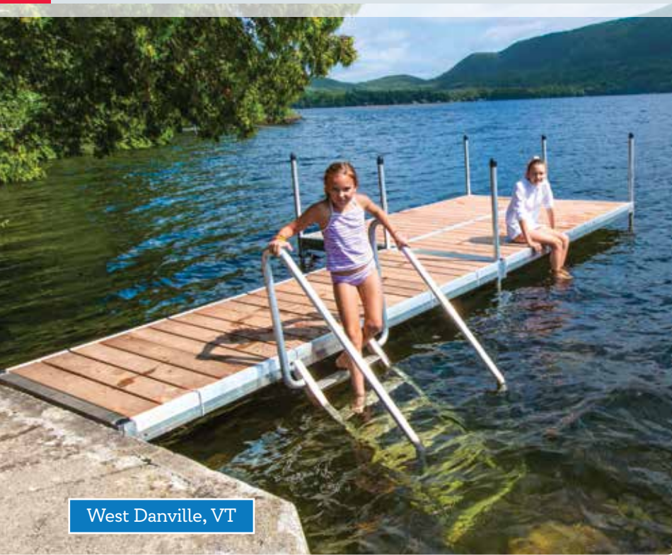
Standard duty aluminum leg dock with cedar decking and our shallow water stairs (see page 18).
