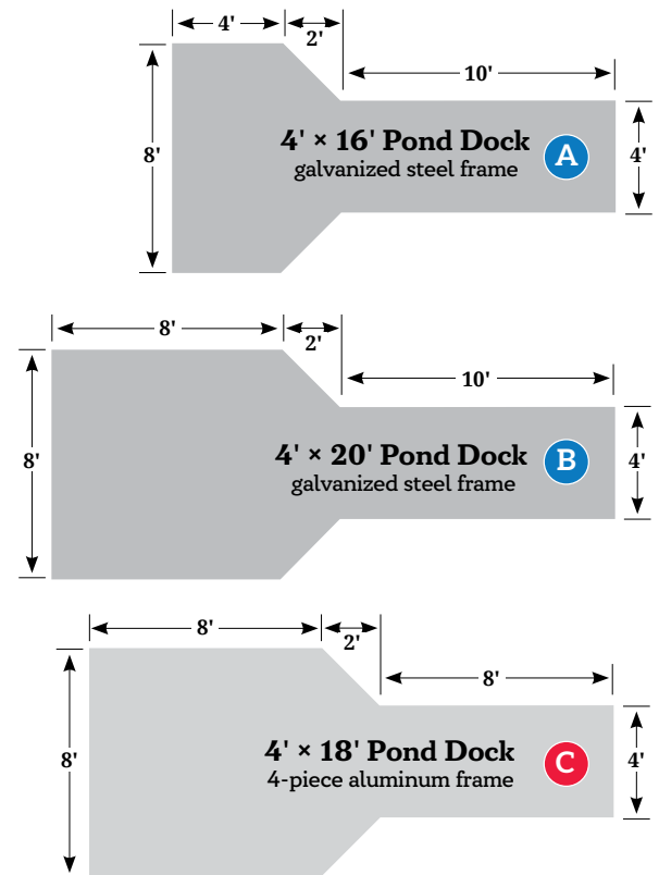
C 4' x 18' Pond Dock 4-piece aluminum frame
