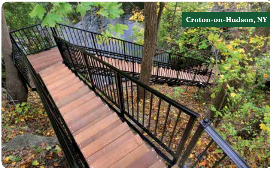
Above & Right: Free span stairs with black powder coating and Ipe treads traversing a vertical drop of approximately 60 feet.
