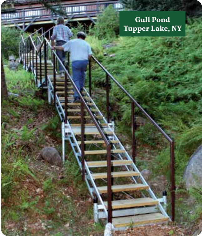
Stairs designed for a gradual, sloping site with brown powder-coated aluminum rails.
