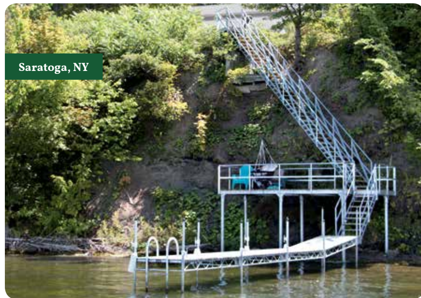
Free span stair system with our shoreside platform as a landing.
