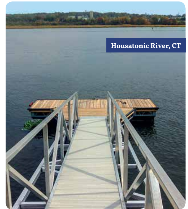
Galvanized steel truss floating dock with vertical fenders & our permanent pile system to allow access when water level is high.
